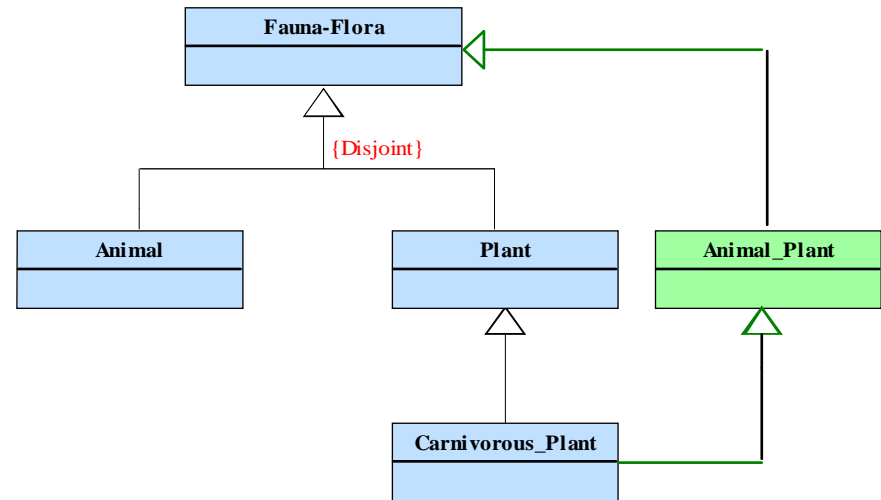
Logical Pattern Instantiation
