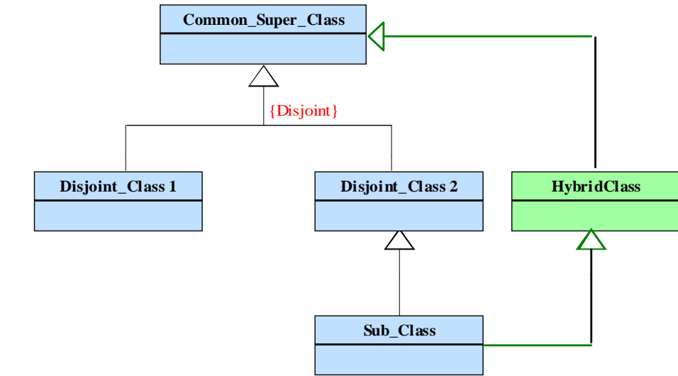
Logical Pattern Solution
